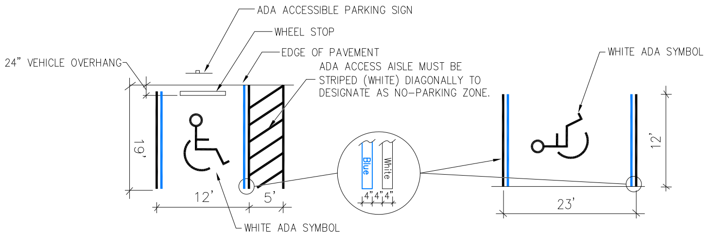
HORIZONTAL PARKING DETAIL
