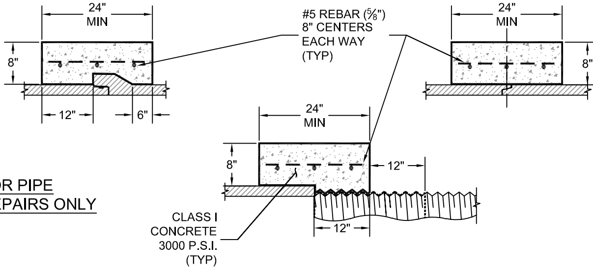
CONCRETE COLLAR SECTIONS
