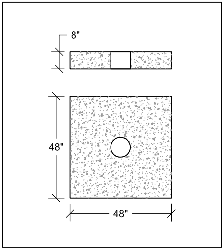
CONCRETE COLLAR DETAIL
