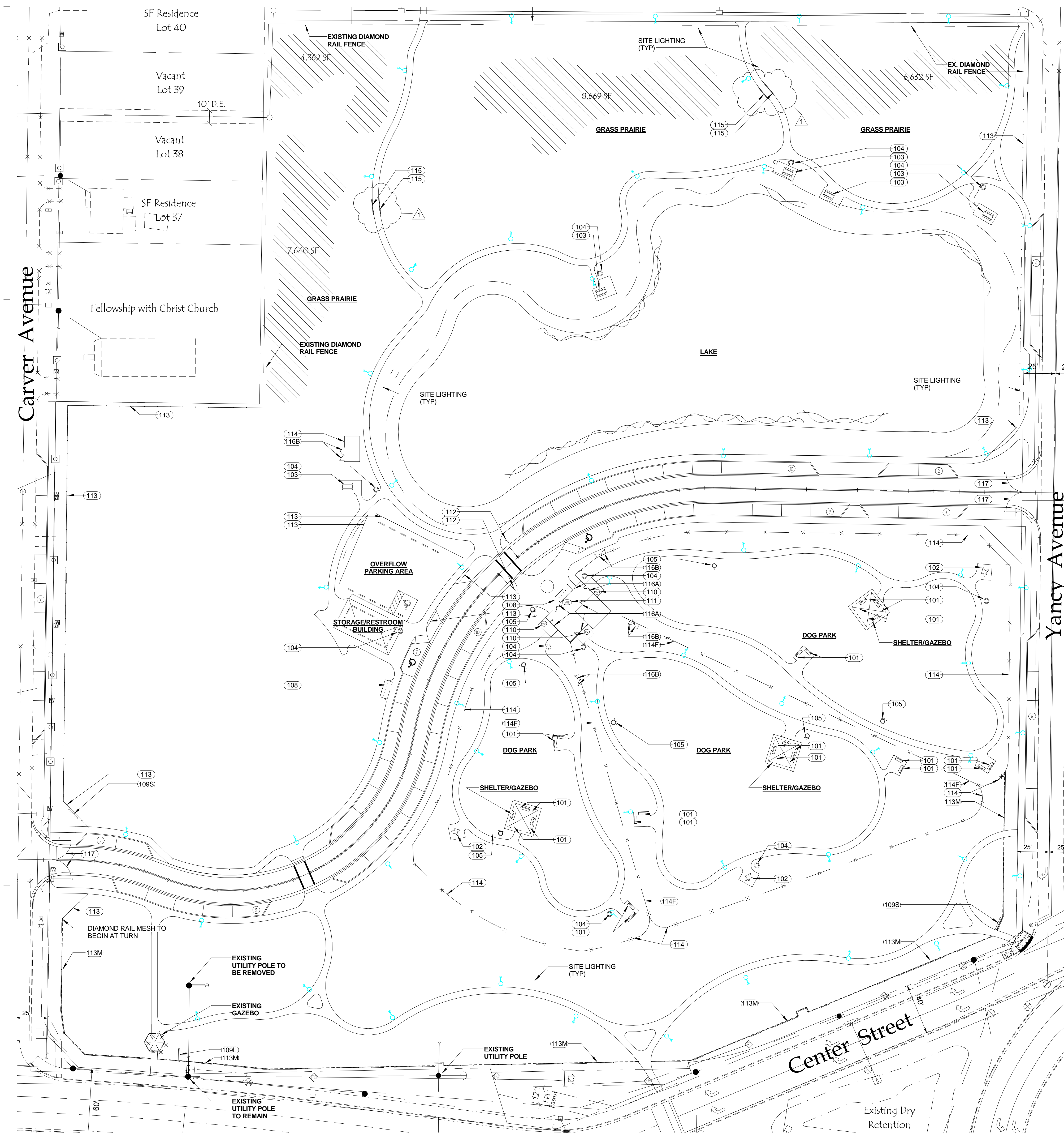
A SITE FURNITURE PLAN AS-2.00 1" = 40'-0"
